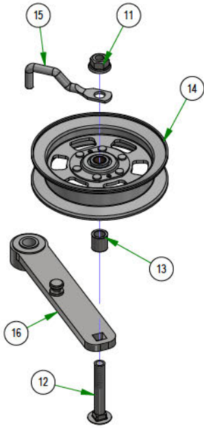
039-6945-26 Maverick HD & Down Deck Idler Assembly
