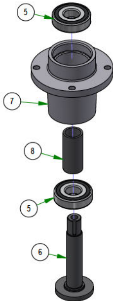
037-2000-00 Spindle Assembly-MZ
