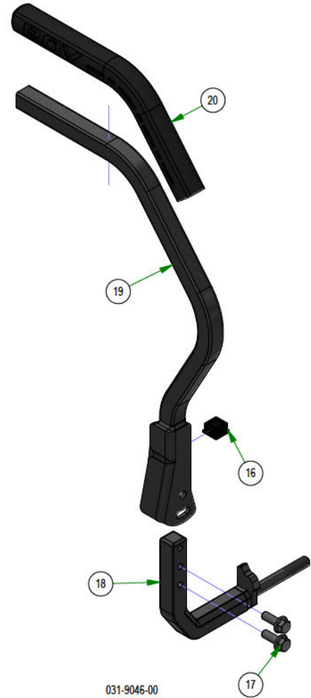
031-9046-00 Small Mower Square Drive Arm LH Assembly
