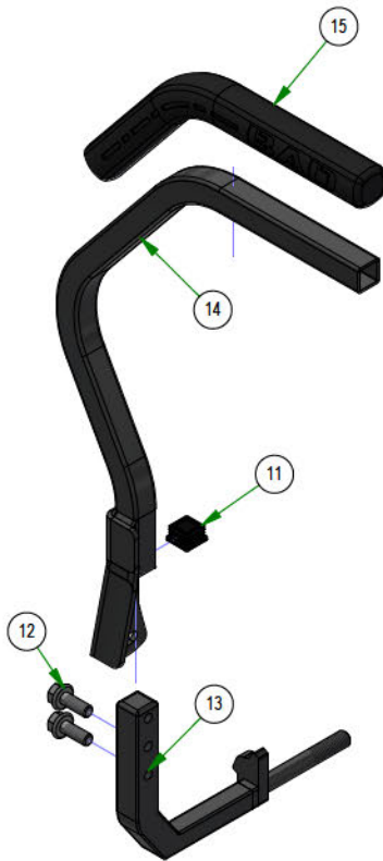
031-9045-00 Small Mower Square Drive Arm RH Assembly
