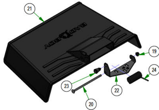
210-6007-00 Plastic Chute Assembly 42" Deck
