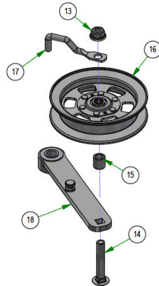
039-6945-26 Maverick HD & Down Deck Idler Assembly
