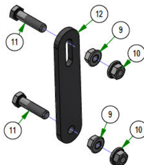
039-2127-17 Deck Hanger Assembly
