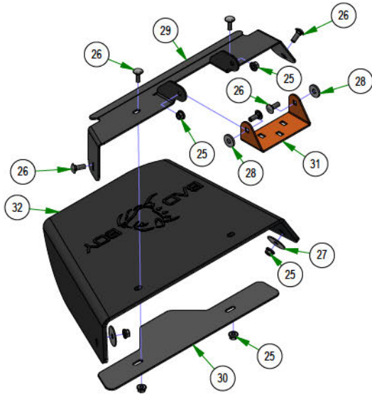
210-6015-98 MZ Discharge Chute Assembly 48", 54", & 60" Decks
