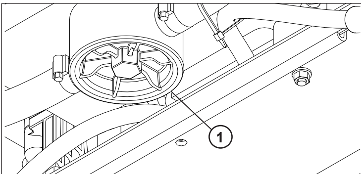
1. Hydraulic filter
