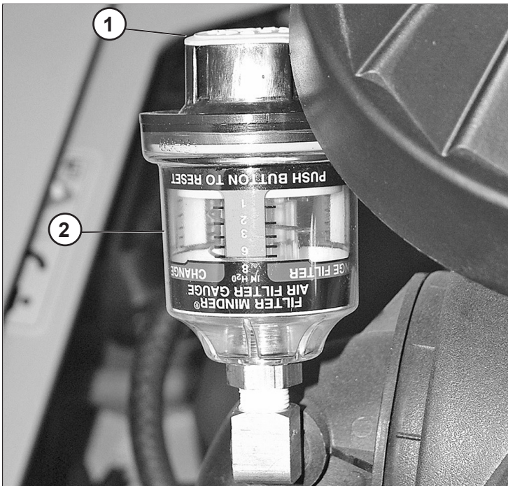
1. Reset button
