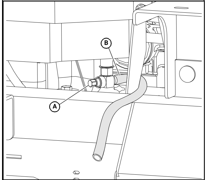
A. Oil drain cap
