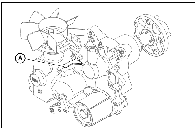
A. Bypass valve lever - open
