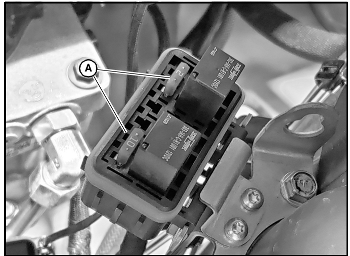
A. Kawasaki EFI engine fuses
